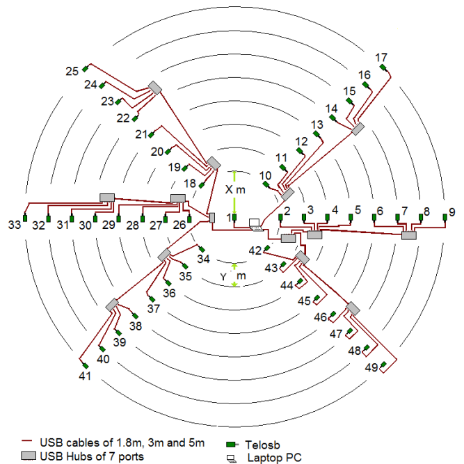
Fig. 1. Nodes distribution according the radial topology.
