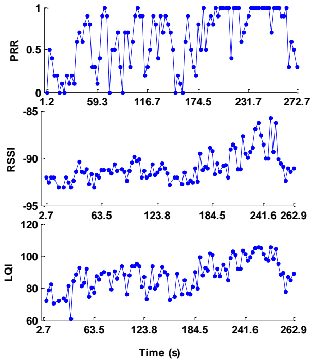
Fig. 6. Temporal behaviour (refer to TABLE 1— Scenario 4).
