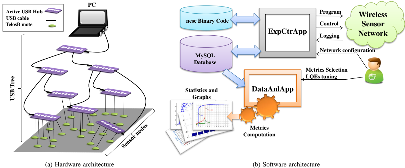
Fig. 2. Testbed Hardware and Software architectures.
