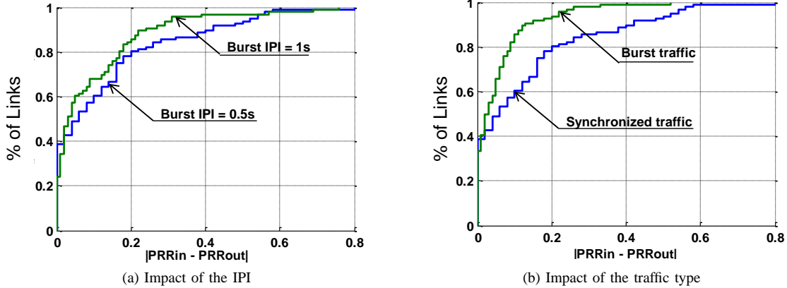
Fig. 7. CDF of the link symmetry level, for different traffic patterns. Synchronized traffic is the most appropriate pattern for the link symmetry level assessment. Bursty traffic can be used for the link symmetry level assessment but with small IPI. (refer to TABLE 1— Scenario 1).
