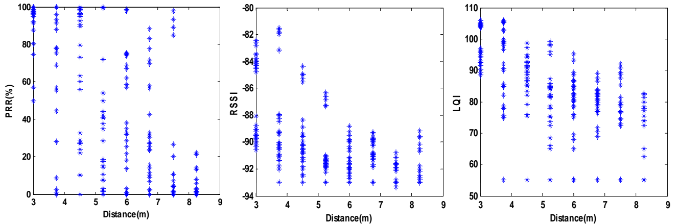
Fig. 5. Spatial behaviour. Two receivers placed at the same distance from the sender may have different link qualities. Moreover, a receiver that is farther from the sender can have better link quality than another receiver nearer to the sender (refer to TABLE I— Scenario 4).
