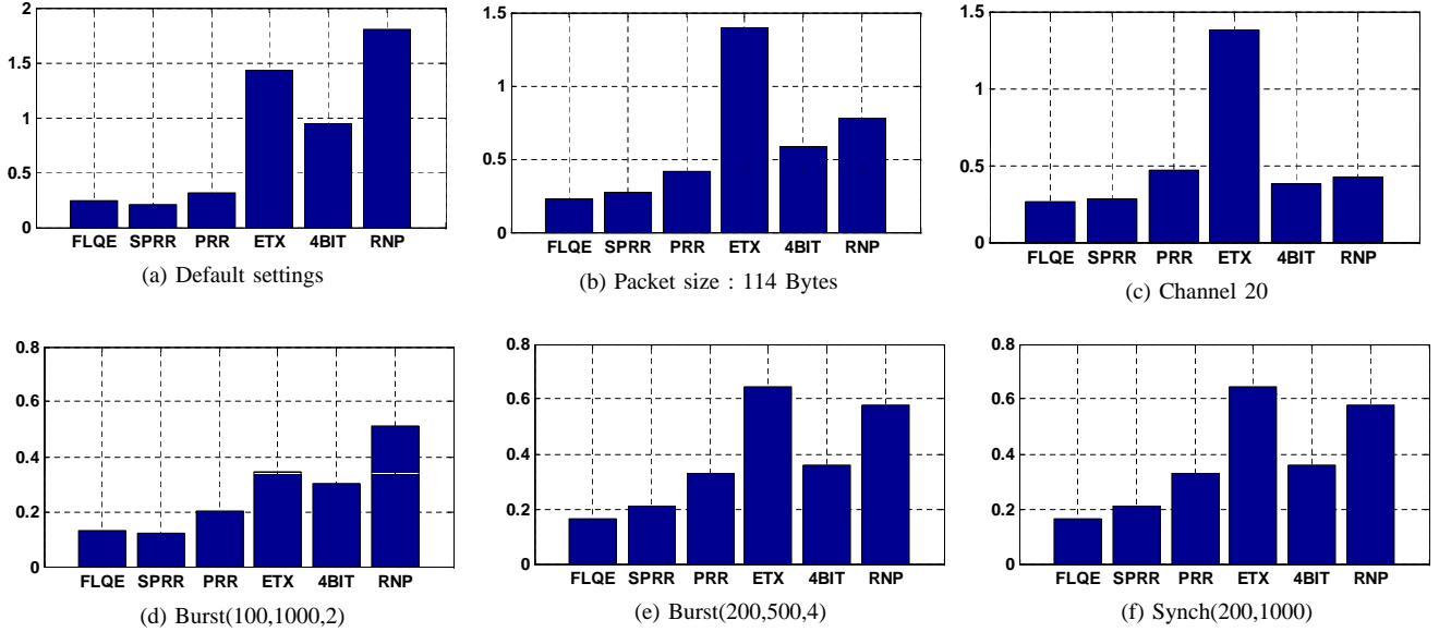
Fig. 11. Stability of LQEs, for different network settings (refer to TABLE 1— Scenarios 1,2,...5).
