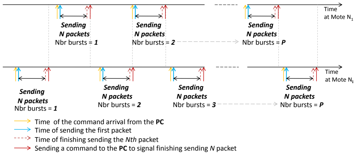
(a) Burst(N, IPI, P) traffic. After receiving the command from the PC, the mote sends a burst of N packets to the other mote, with an inter-packet interval equal to IPI seconds. This operation is repeated until reaching a total number of sent bursts equal to P
