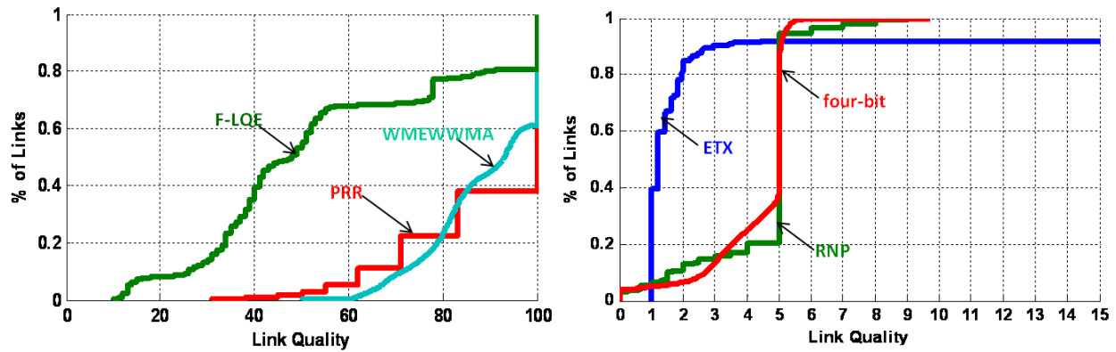
Fig. 13. Empirical CDFs of LQEs, based on all the links in the simulated network (Tossim 2 simulation results).
