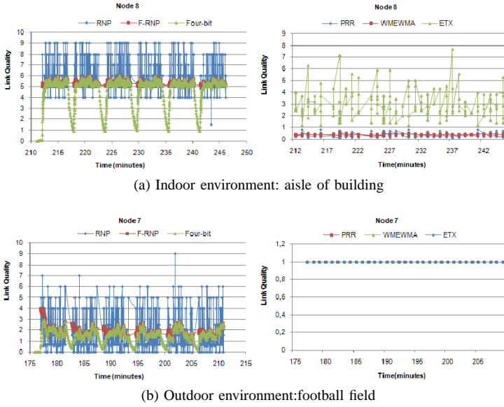
Fig. 6. Temporal behaviour of link quality estimators (Traffic Pattern 1, w = 5 )
