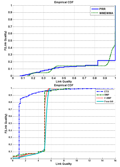
Fig. 7. Empirical CDFs of link quality estimators (Traffic Pattern 1, Indoor environment, w = 5 )
