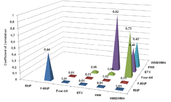
Fig. 9. Correlation between link quality estimators (Traffic Pattern 2, Indoor environment, w = 5 )
